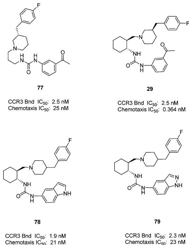
Figure 2. Chemotaxis SAR of compounds discussed in text.
